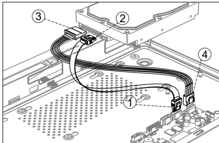
Figure 1-11 Connect Cables
