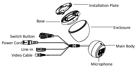
Figure 1-10 Overview of Type V Camera (DF8T Series)
