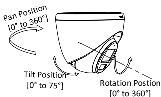
Figure 2-9 3-Axis Adjustment
