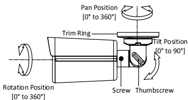
Figure 2-2 3-Axis Adjustment
